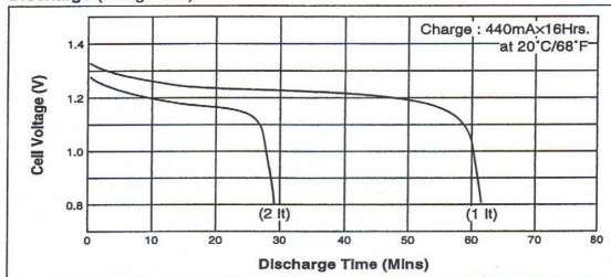
Discharge (at high rate)
